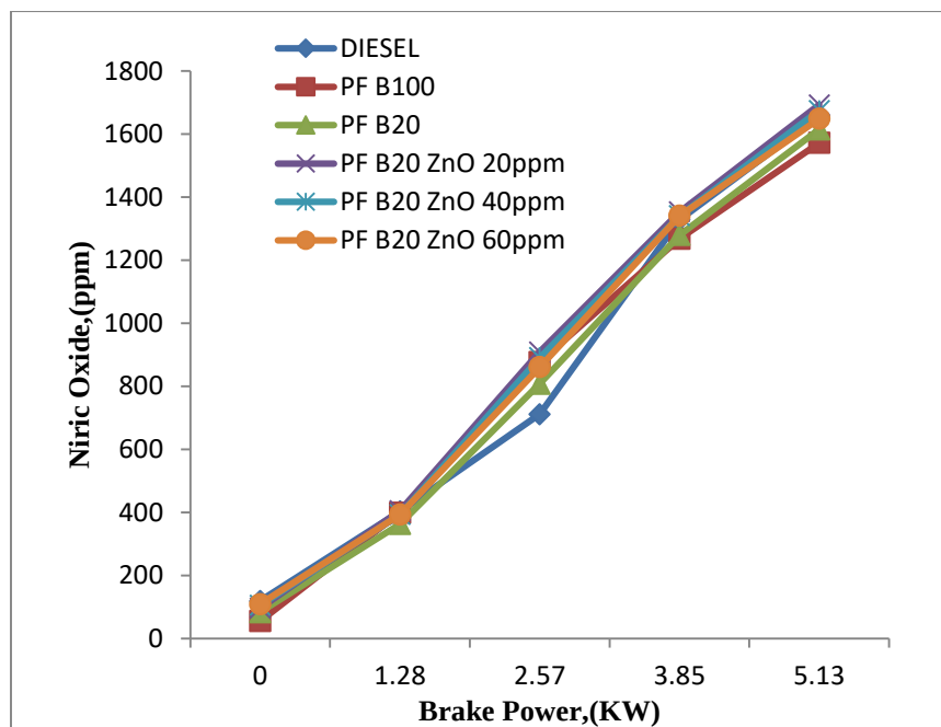
Fig 4.4 Brake power Vs Nitric Oxides
