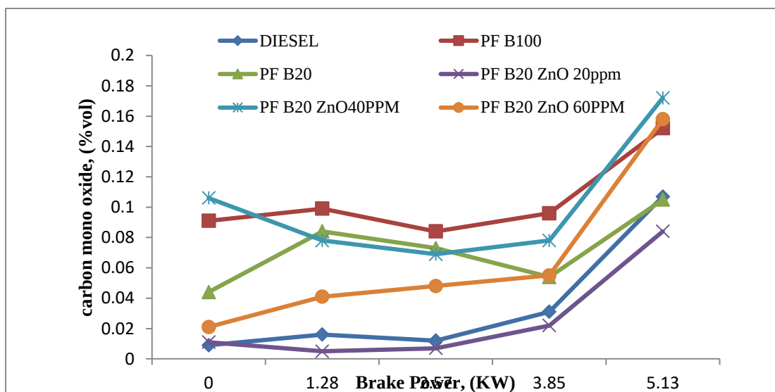
Fig 4.1 Brake power Vs carbon monoxide
