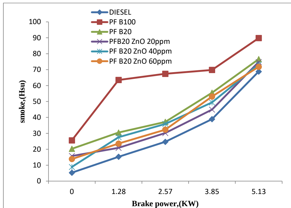
Fig 4.5 Brake power Vs Smoke
