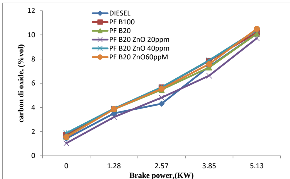
Fig 4.2 Brake power Vs carbon dioxide
